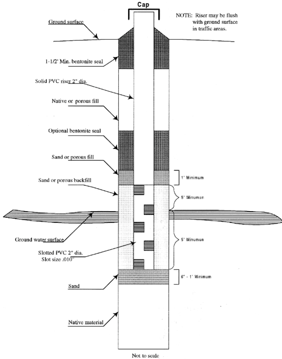
VERTICAL MONITORING WELL
